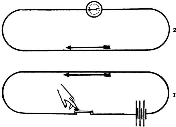
FIG. 288.—Diagram Illustrating the Action of Voltaic Induction Between Two Circuits: the one including a source of electrical energy and a switch; the other including a galvanometer, but having no cell or other electrical source. The direction of the battery current in circuit 1 is indicated by the arrow; the arrow in circuit 2 showing the direction of the induced current.
